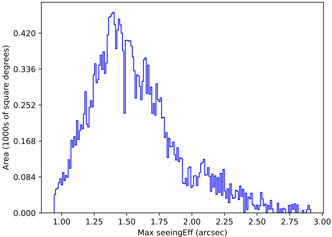
extra_ss_neo7_v3.4_10yrs Yr 1 i band: Max seeingEff
