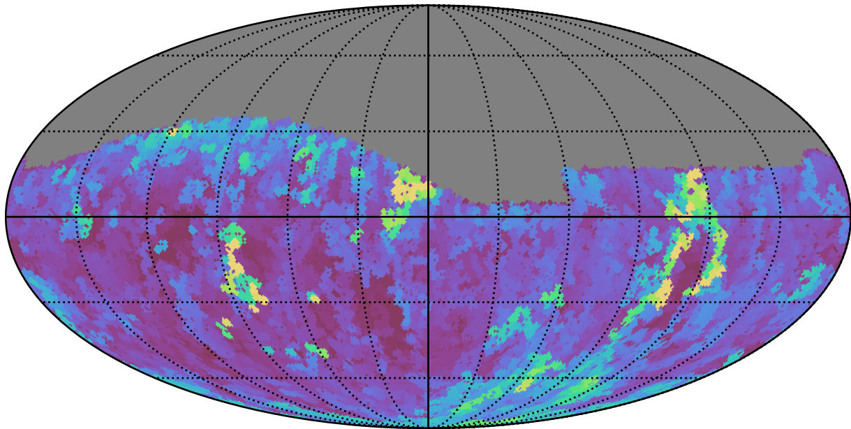
extra_ss_neo7_v3.4_10yrs Yr 1 g band: Max seeingEff
