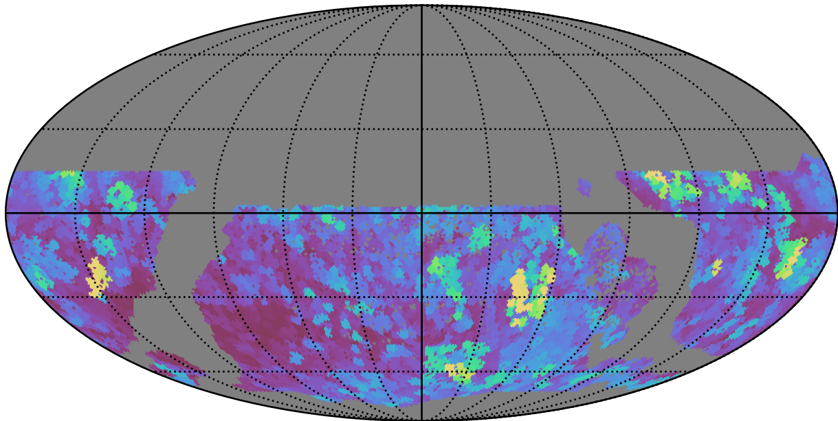
extra_ss_neo7_v3.4_10yrs WFD z band: Max seeingEff
