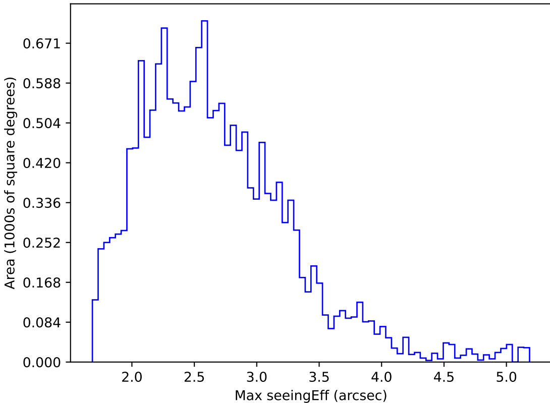
extra_ss_neo7_v3.4_10yrs WFD z band: Max seeingEff
