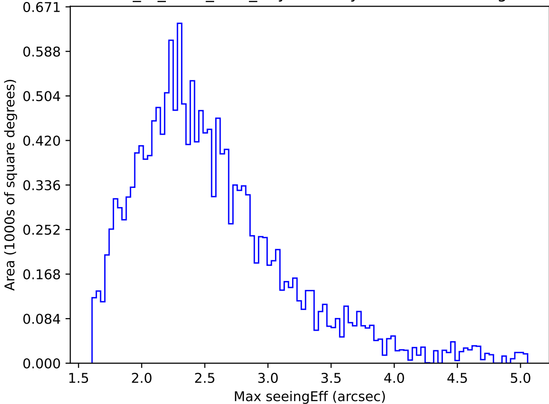
extra_ss_neo7_v3.4_10yrs WFD y band: Max seeingEff
