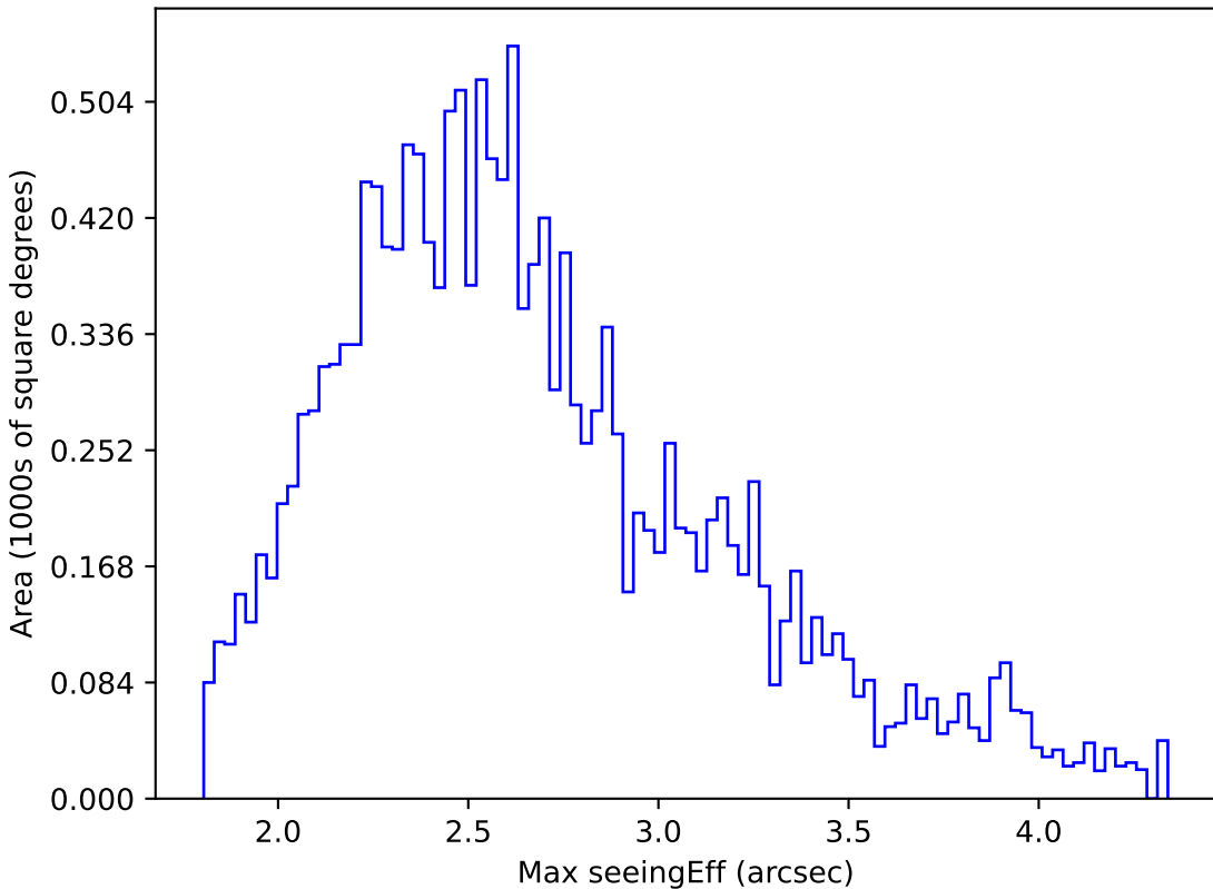
extra_ss_neo7_v3.4_10yrs WFD r band: Max seeingEff
