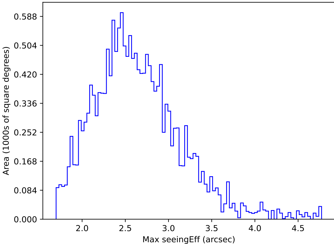
extra_ss_neo7_v3.4_10yrs WFD i band: Max seeingEff
