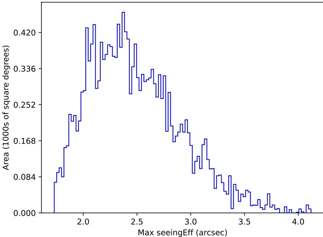
extra_ss_neo7_v3.4_10yrs WFD g band: Max seeingEff
