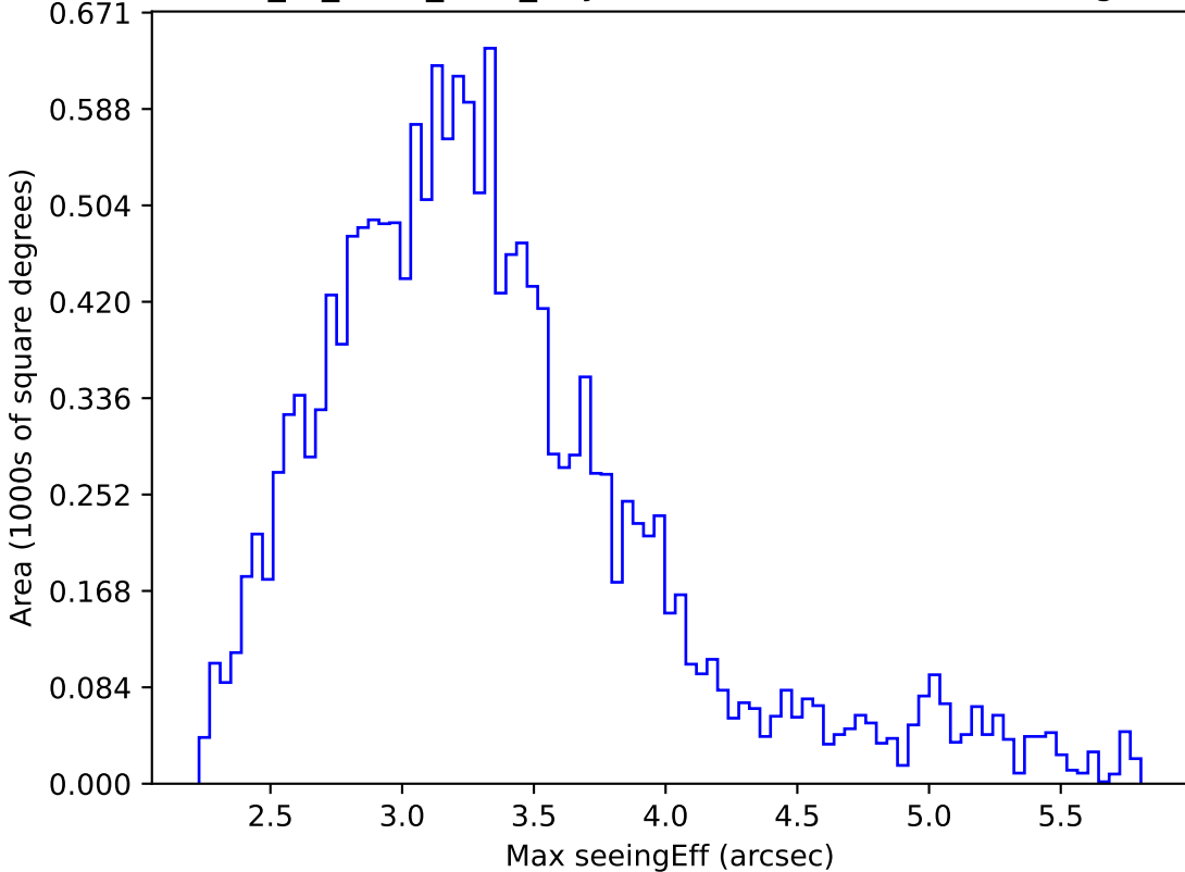
extra_ss_neo7_v3.4_10yrs WFD all bands: Max seeingEff
