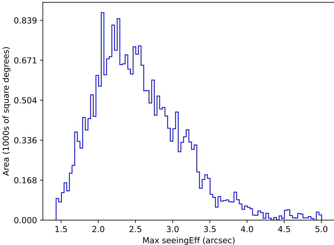
extra_ss_neo7_v3.4_10yrs All sky z band: Max seeingEff
