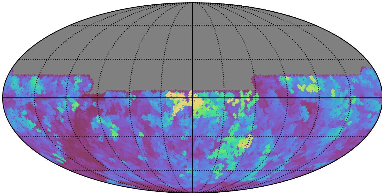
extra_ss_neo7_v3.4_10yrs All sky y band: Max seeingEff
