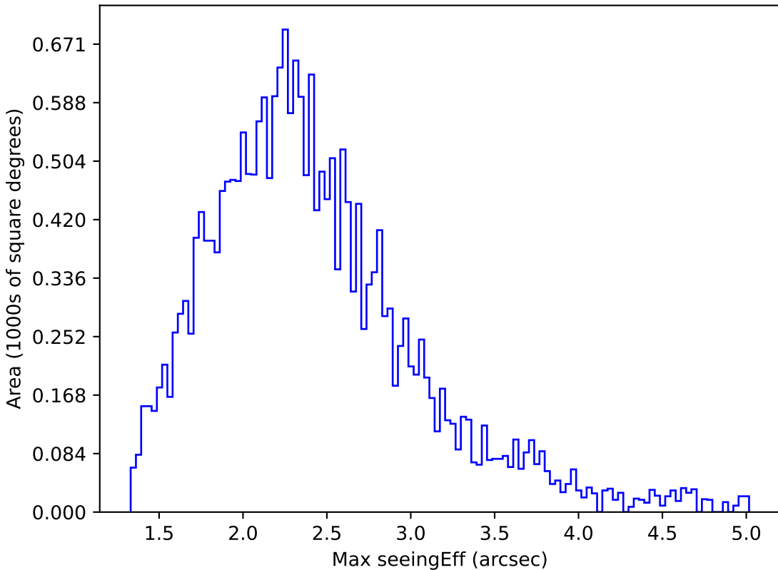
extra_ss_neo7_v3.4_10yrs All sky y band: Max seeingEff
