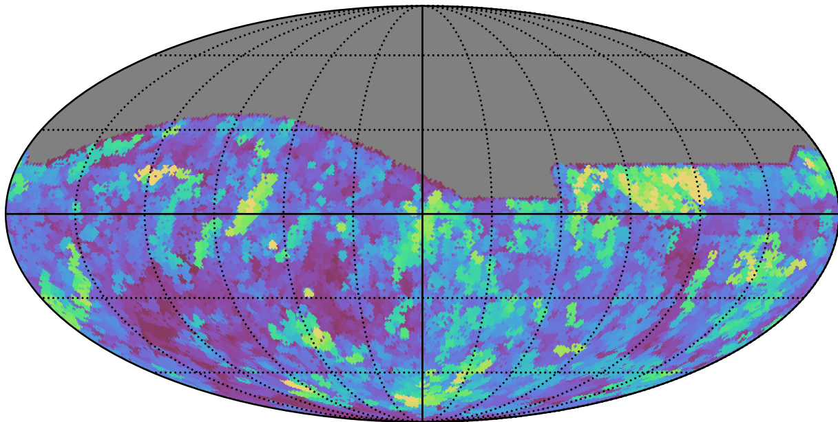
extra_ss_neo7_v3.4_10yrs All sky r band: Max seeingEff
