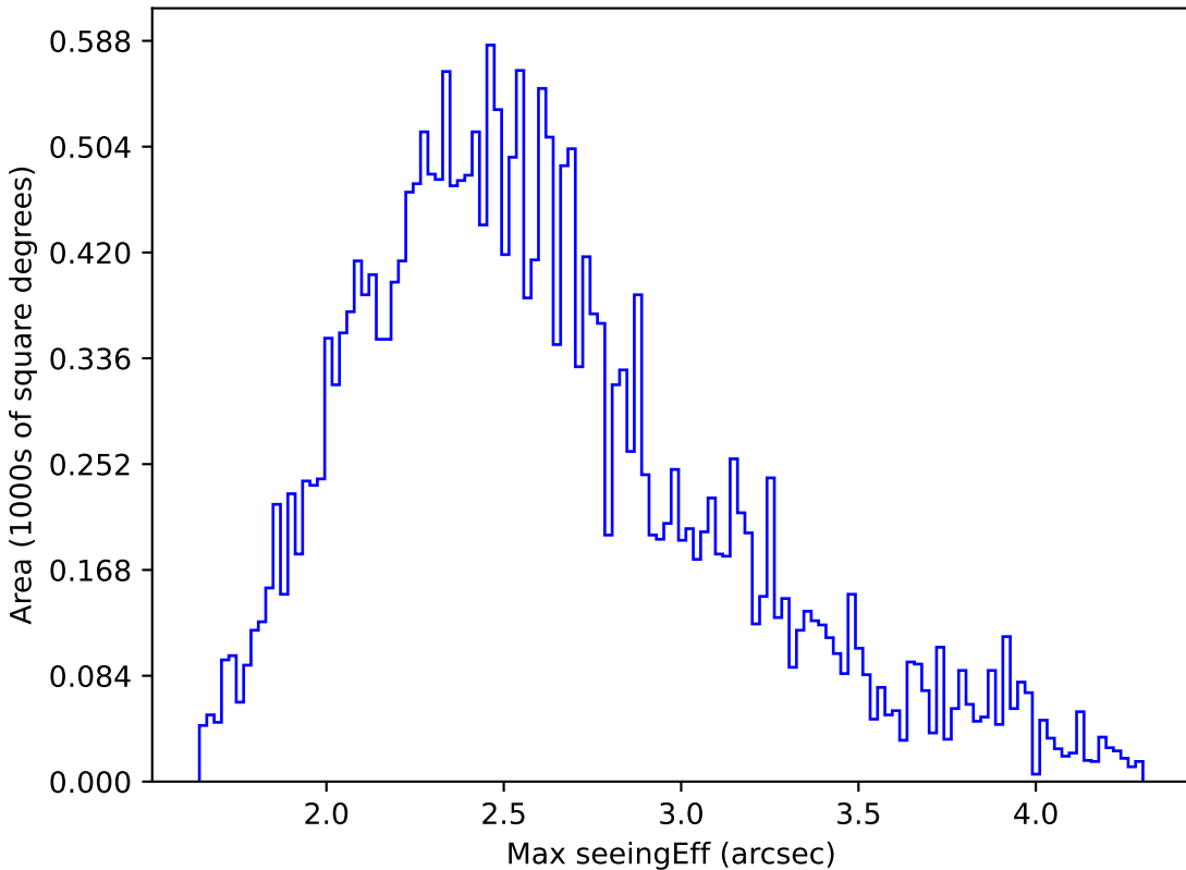
extra_ss_neo7_v3.4_10yrs All sky r band: Max seeingEff
