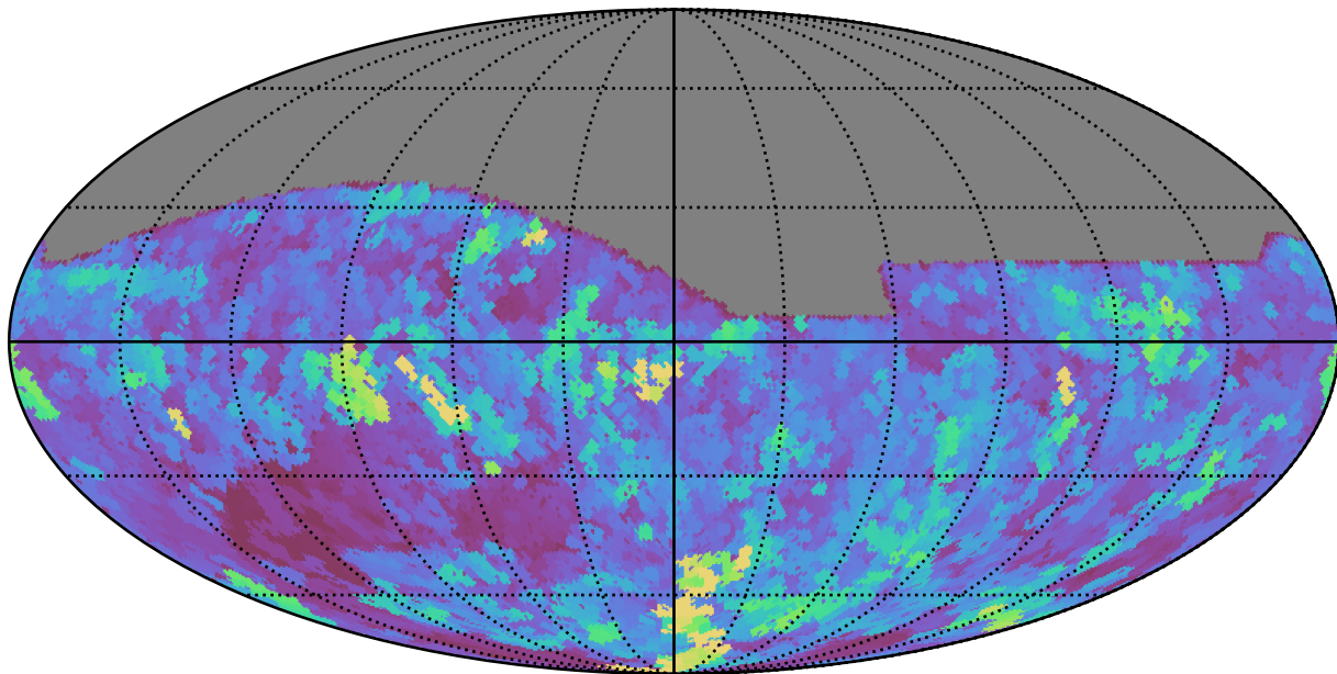
extra_ss_neo7_v3.4_10yrs All sky i band: Max seeingEff
