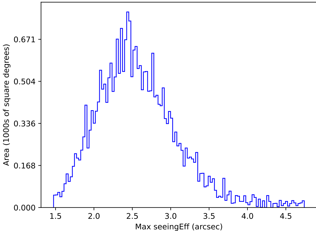
extra_ss_neo7_v3.4_10yrs All sky i band: Max seeingEff
