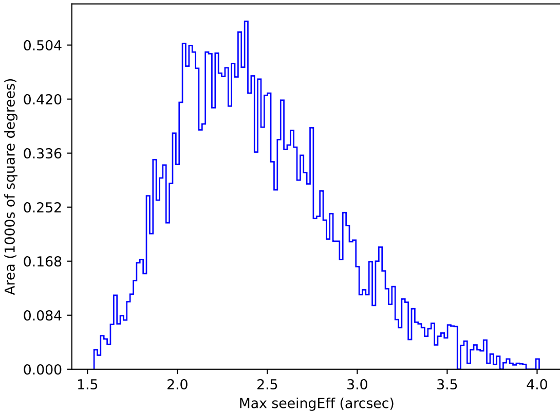
extra_ss_neo7_v3.4_10yrs All sky g band: Max seeingEff
