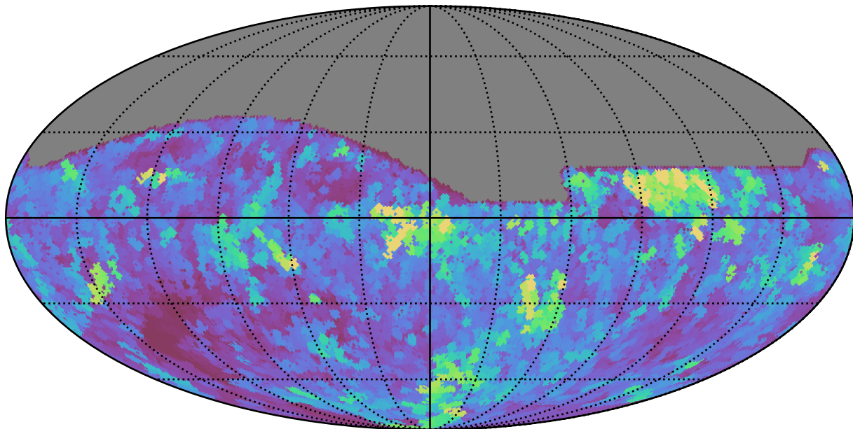
extra_ss_neo7_v3.4_10yrs All sky all bands: Max seeingEff
