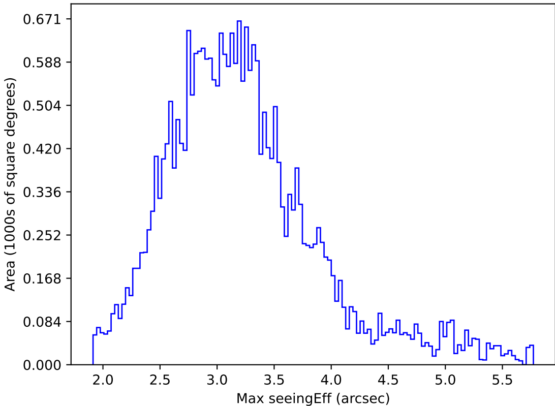
extra_ss_neo7_v3.4_10yrs All sky all bands: Max seeingEff
