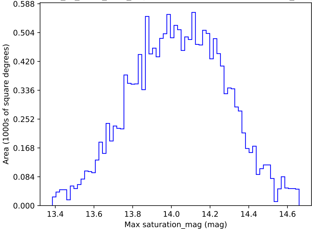
extra_ss_neo7_v3.4_10yrs WFD u band: Max saturation_mag
