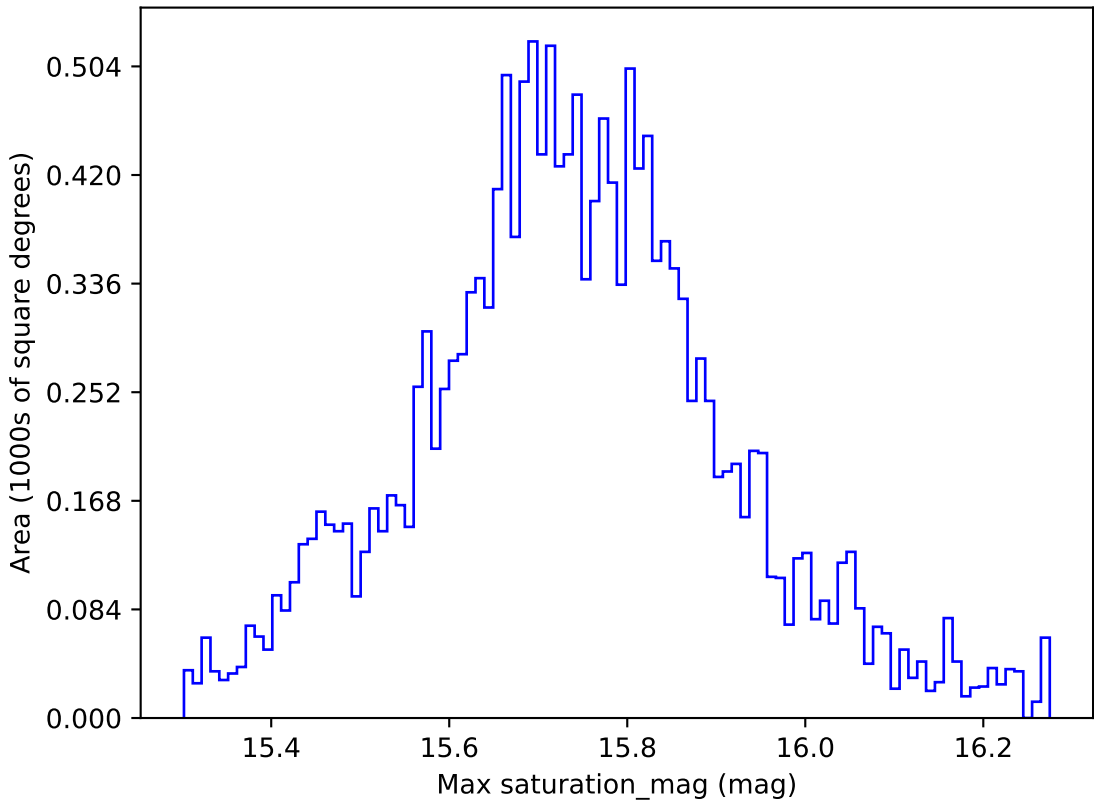
extra_ss_neo7_v3.4_10yrs WFD g band: Max saturation_mag
