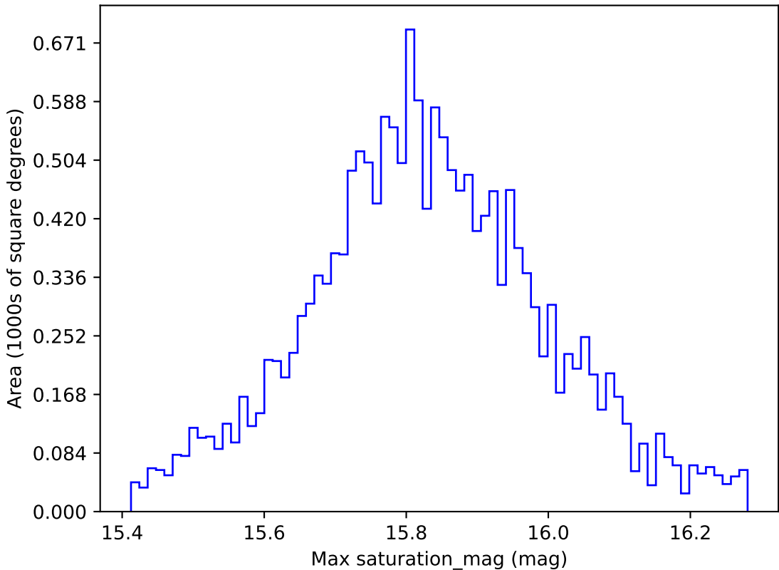
extra_ss_neo7_v3.4_10yrs WFD all bands: Max saturation_mag
