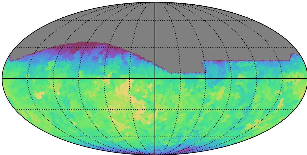
extra_ss_neo7_v3.4_10yrs All sky all bands: Max saturation_mag
