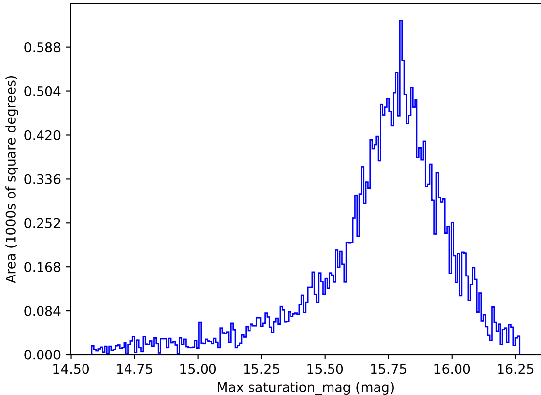
extra_ss_neo7_v3.4_10yrs All sky all bands: Max saturation_mag
