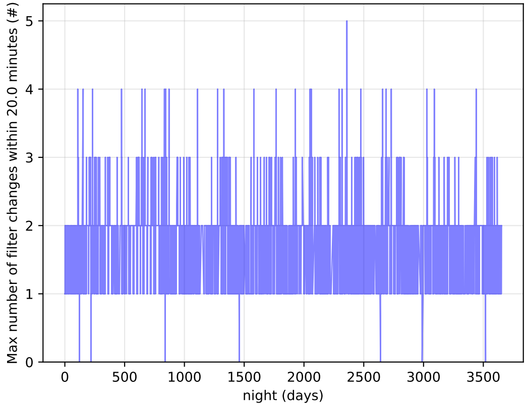
extra_ss_neo7_v3.4_10yrs Per Night: Max number of filter changes within 20.0 minutes
