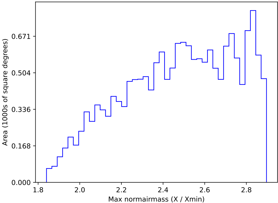
extra_ss_neo7_v3.4_10yrs WFD all bands: Max normairmass
