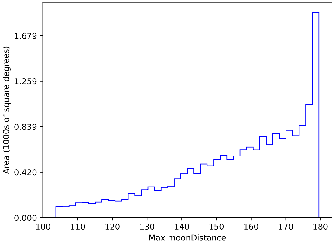
extra_ss_neo7_v3.4_10yrs WFD all bands: Max moonDistance
