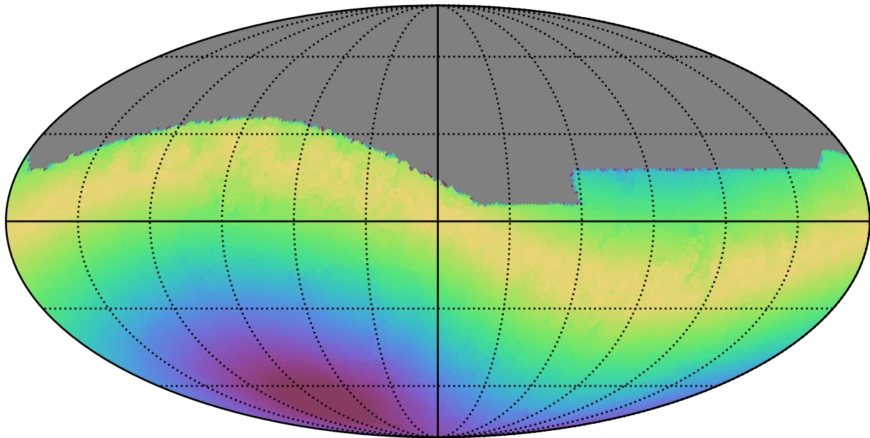
extra_ss_neo7_v3.4_10yrs All sky all bands: Max moonDistance
