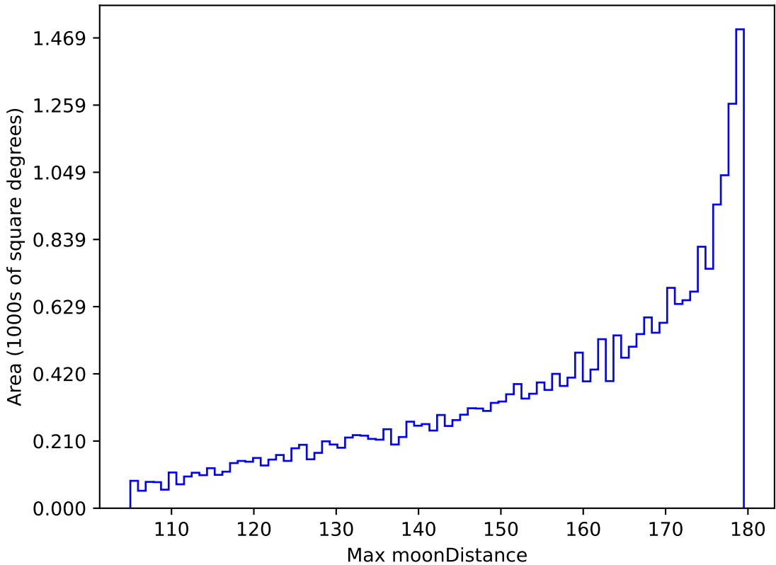
extra_ss_neo7_v3.4_10yrs All sky all bands: Max moonDistance
