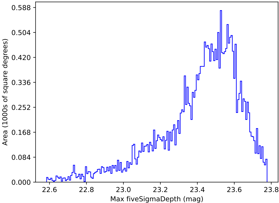
extra_ss_neo7_v3.4_10yrs Yr 1 z band: Max fiveSigmaDepth
