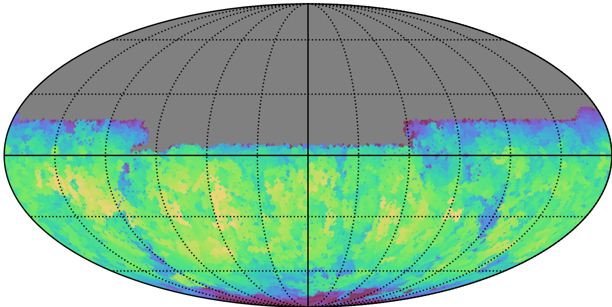
extra_ss_neo7_v3.4_10yrs Yr 1 y band: Max fiveSigmaDepth
