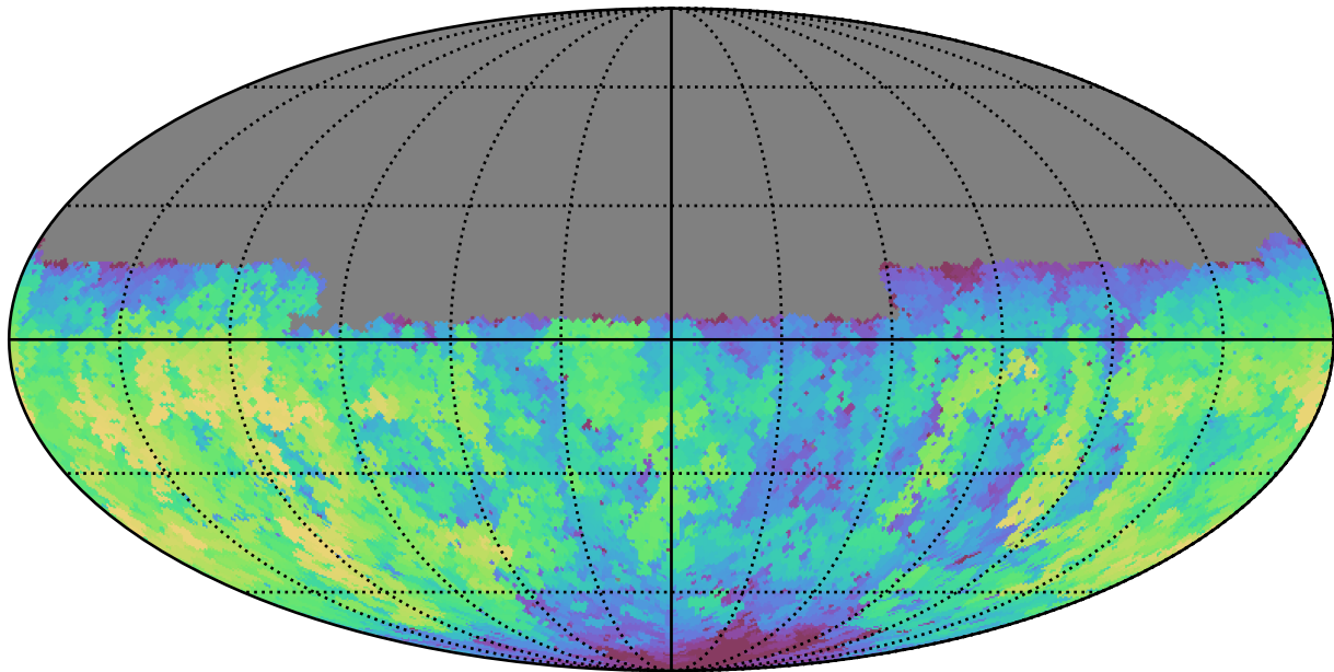
extra_ss_neo7_v3.4_10yrs Yr 1 u band: Max fiveSigmaDepth
