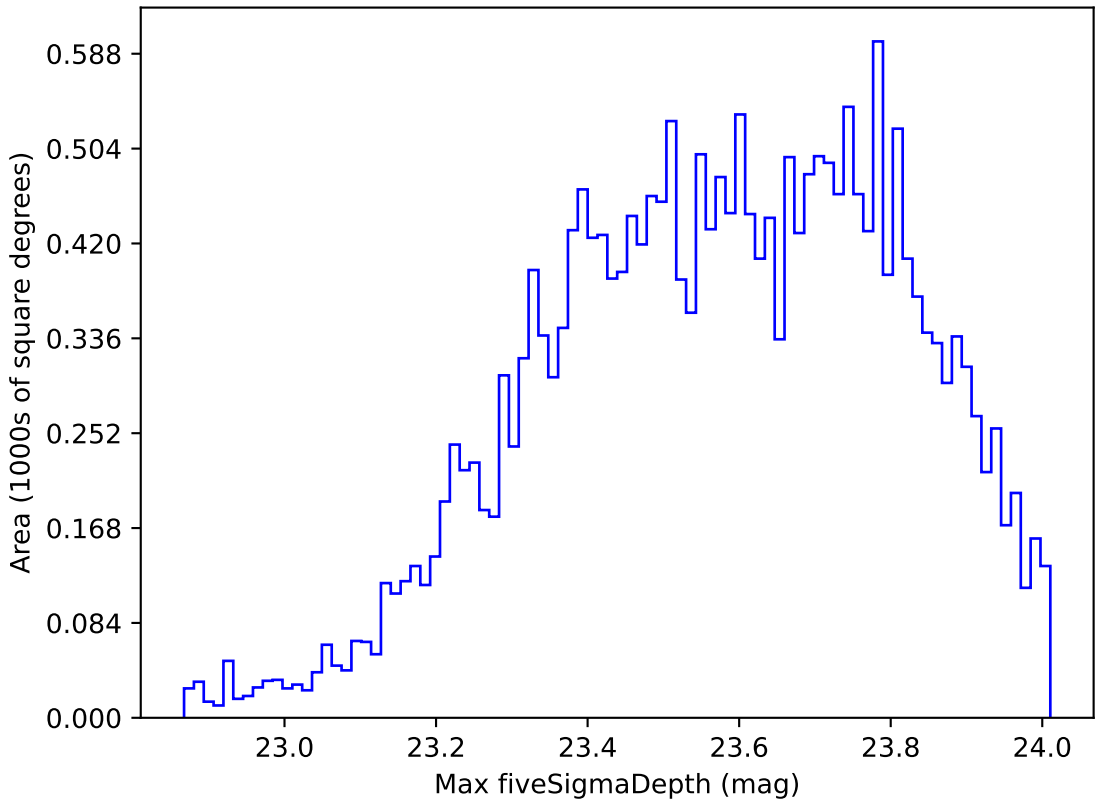
extra_ss_neo7_v3.4_10yrs Yr 1 u band: Max fiveSigmaDepth
