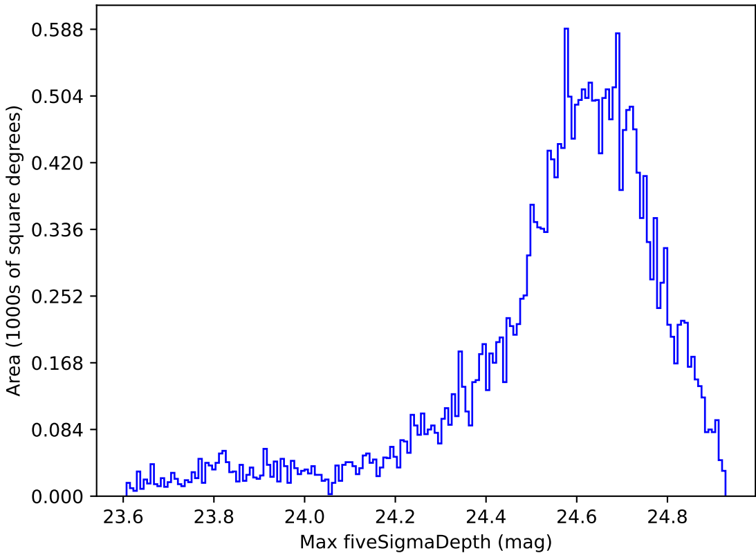
extra_ss_neo7_v3.4_10yrs Yr 1 r band: Max fiveSigmaDepth
