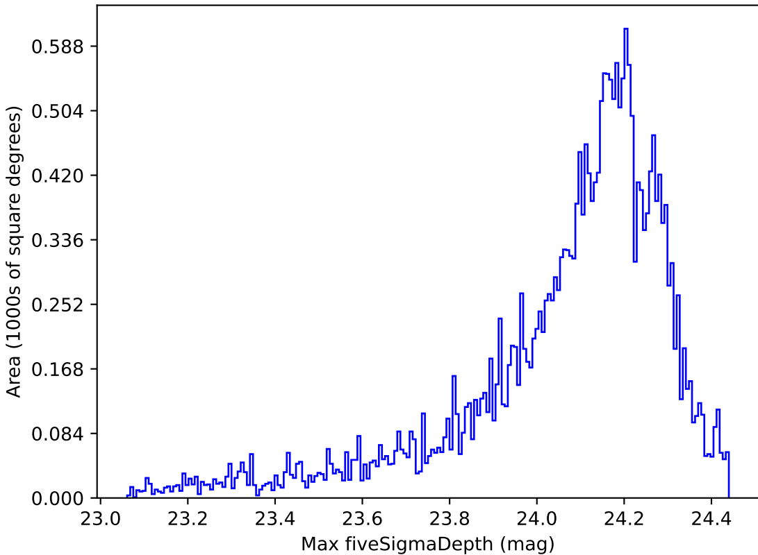
extra_ss_neo7_v3.4_10yrs Yr 1 i band: Max fiveSigmaDepth
