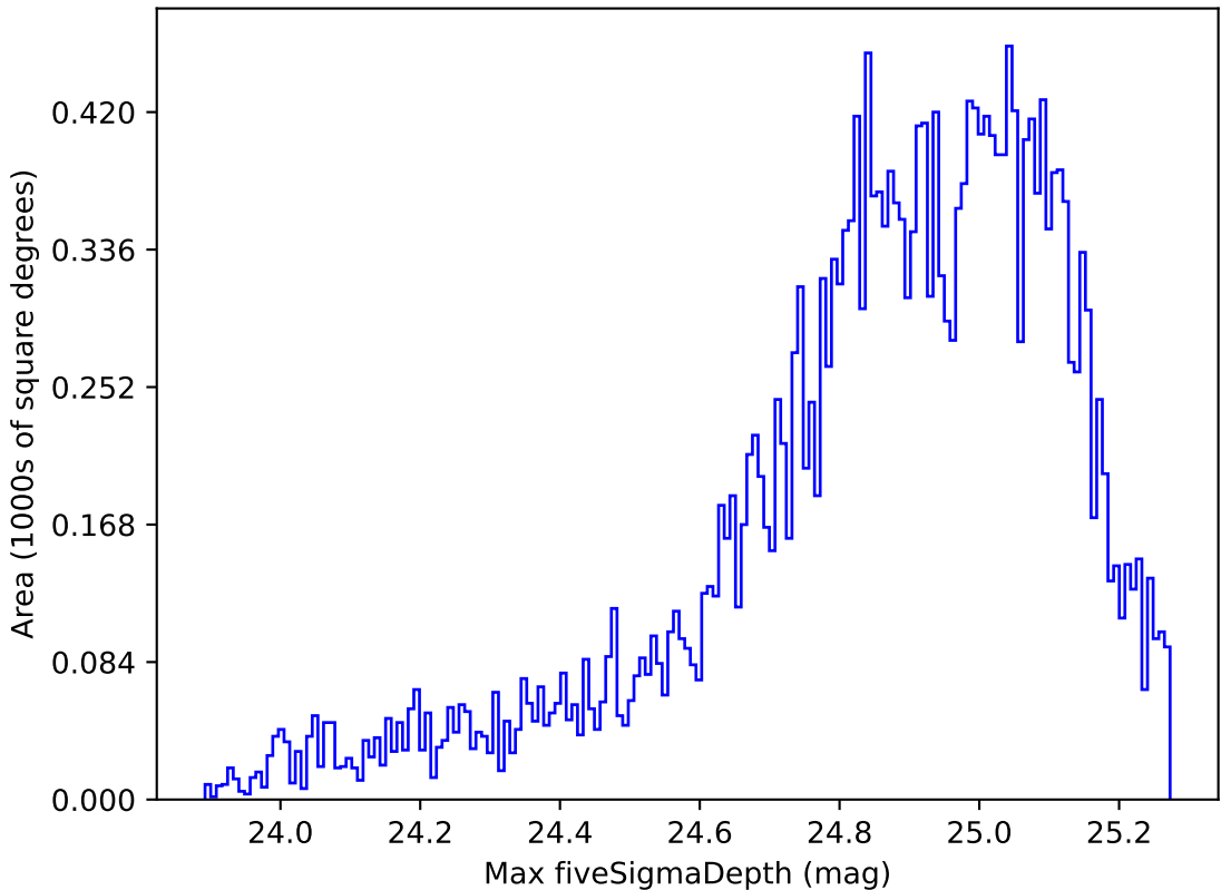
extra_ss_neo7_v3.4_10yrs Yr 1 g band: Max fiveSigmaDepth
