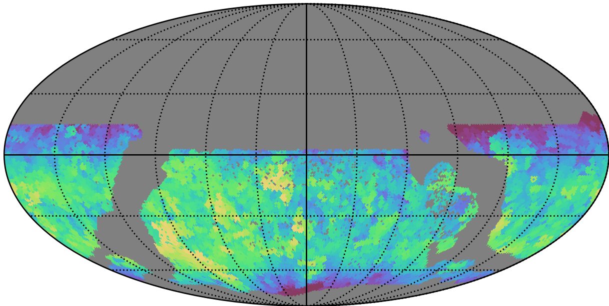
extra_ss_neo7_v3.4_10yrs WFD z band: Max fiveSigmaDepth
