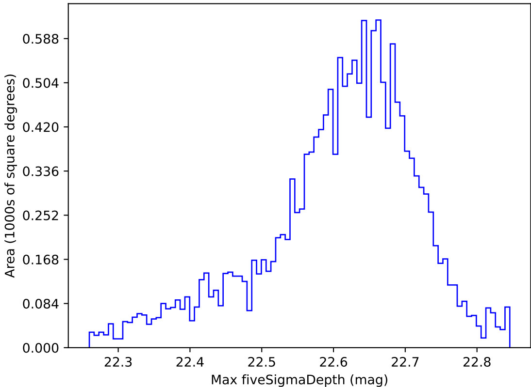
extra_ss_neo7_v3.4_10yrs WFD y band: Max fiveSigmaDepth
