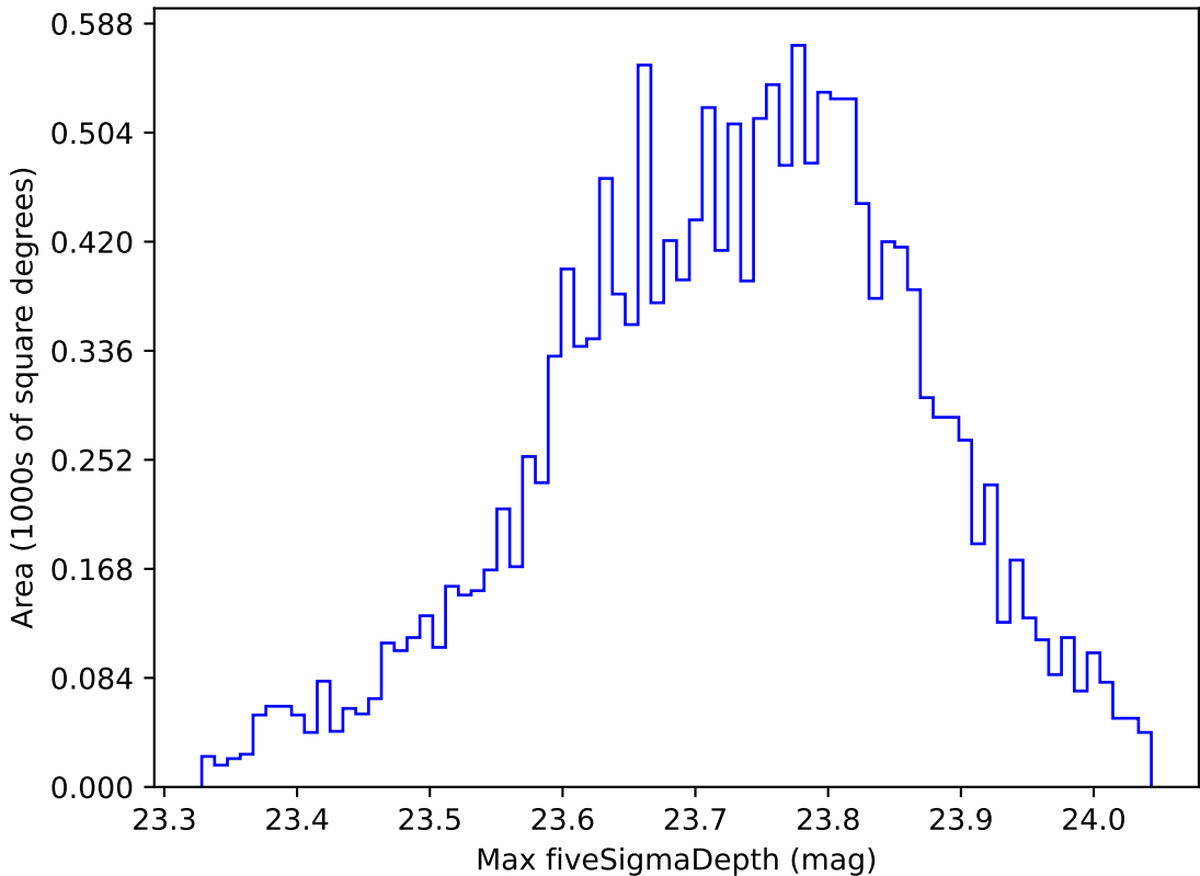
extra_ss_neo7_v3.4_10yrs WFD u band: Max fiveSigmaDepth
