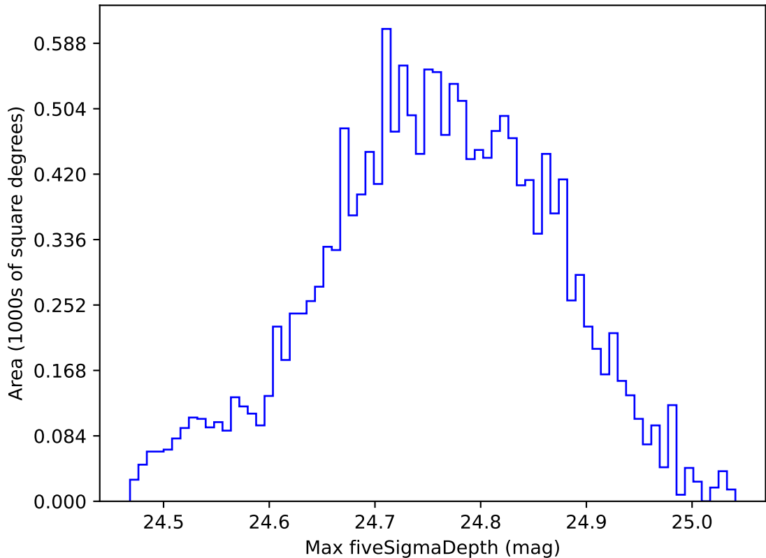
extra_ss_neo7_v3.4_10yrs WFD r band: Max fiveSigmaDepth
