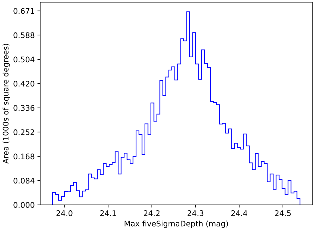
extra_ss_neo7_v3.4_10yrs WFD i band: Max fiveSigmaDepth
