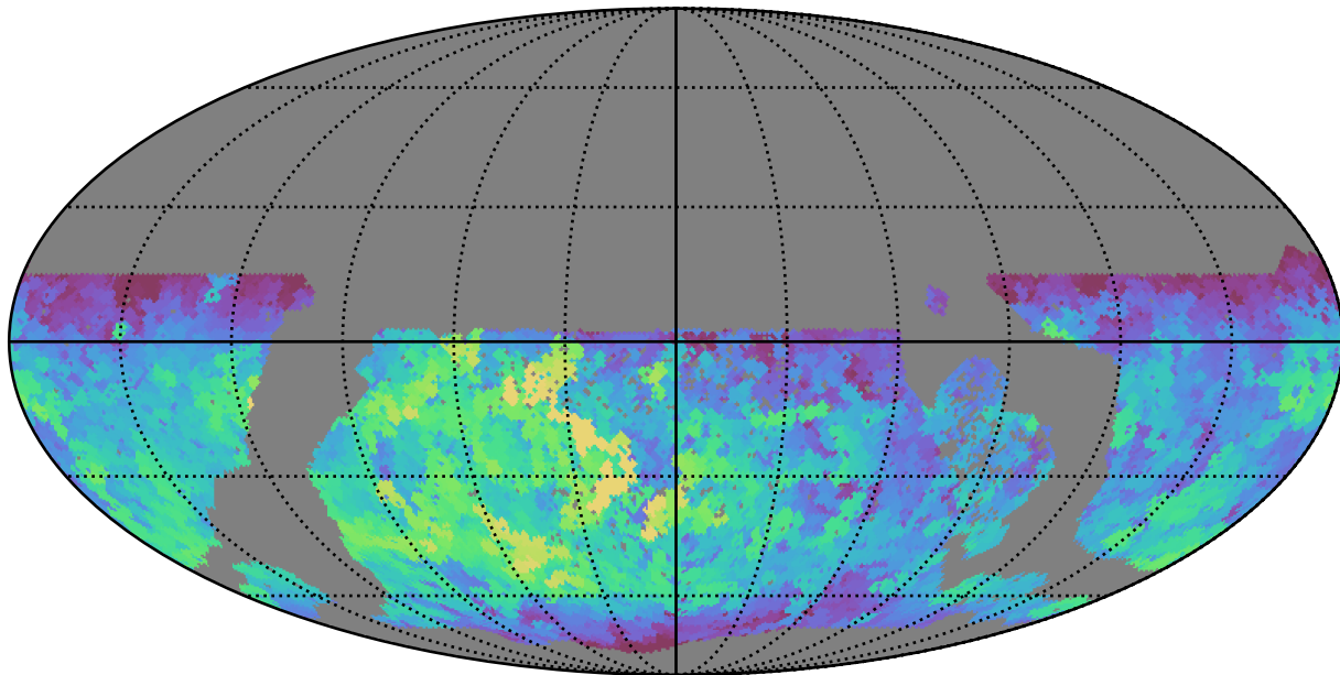
extra_ss_neo7_v3.4_10yrs WFD g band: Max fiveSigmaDepth
