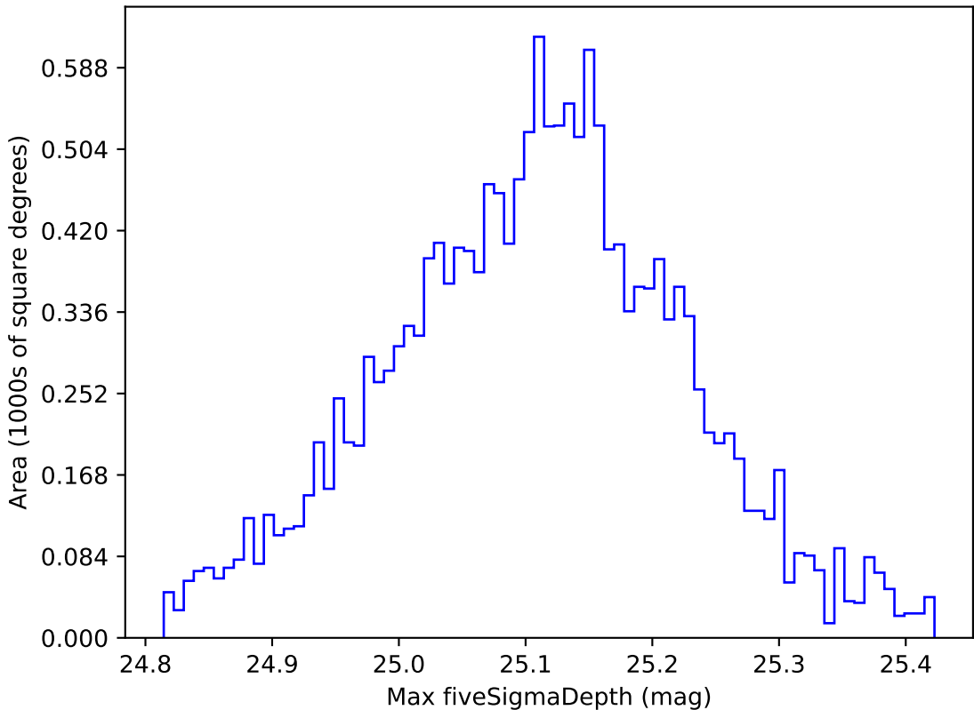
extra_ss_neo7_v3.4_10yrs WFD g band: Max fiveSigmaDepth
