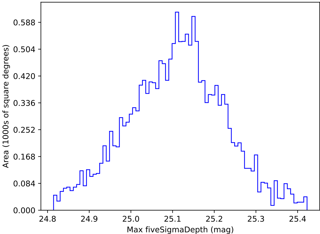
extra_ss_neo7_v3.4_10yrs WFD all bands: Max fiveSigmaDepth
