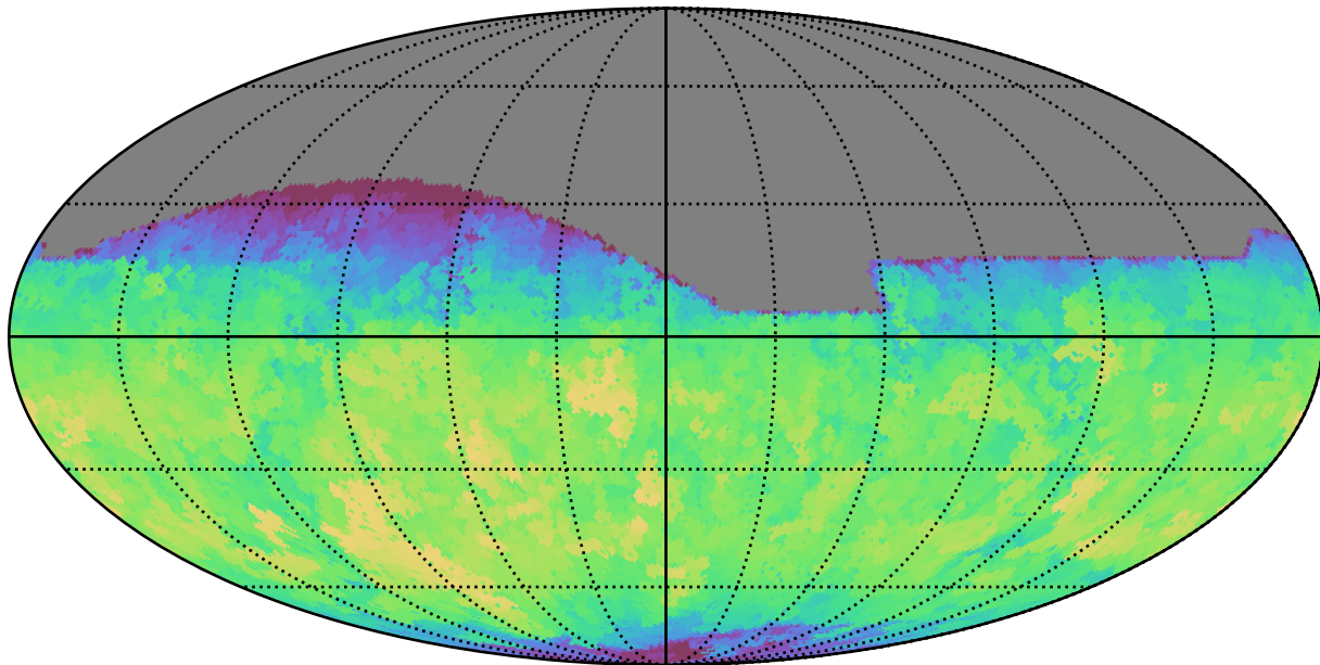
extra_ss_neo7_v3.4_10yrs All sky z band: Max fiveSigmaDepth
