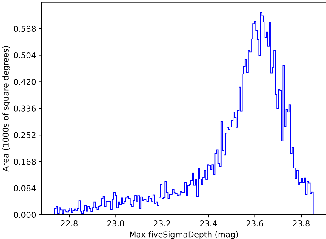
extra_ss_neo7_v3.4_10yrs All sky z band: Max fiveSigmaDepth
