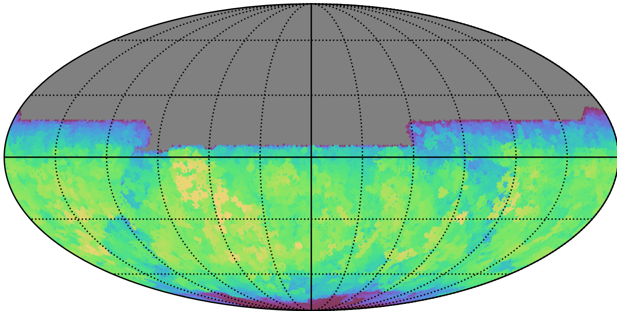
extra_ss_neo7_v3.4_10yrs All sky y band: Max fiveSigmaDepth
