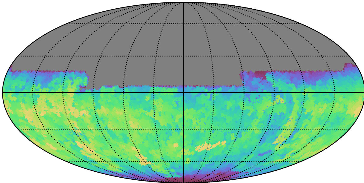
extra_ss_neo7_v3.4_10yrs All sky u band: Max fiveSigmaDepth
