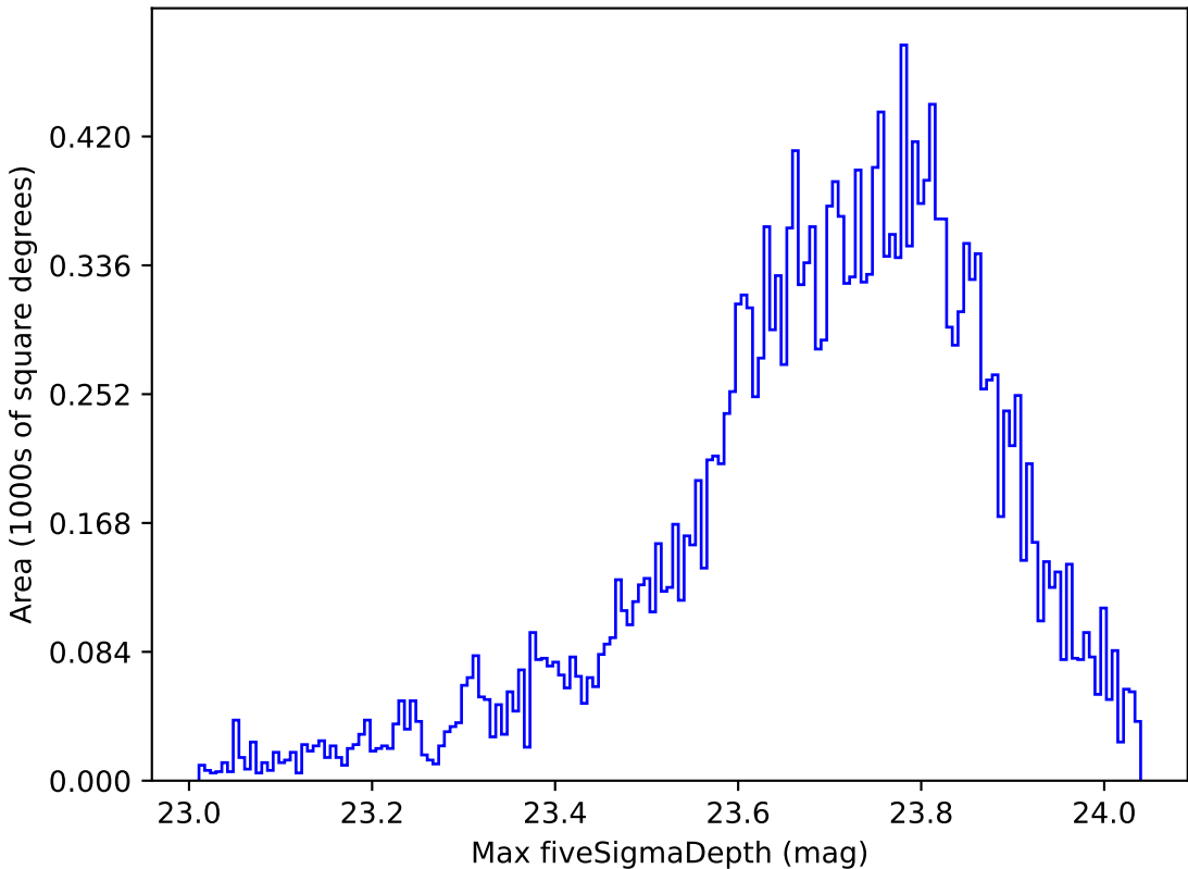
extra_ss_neo7_v3.4_10yrs All sky u band: Max fiveSigmaDepth
