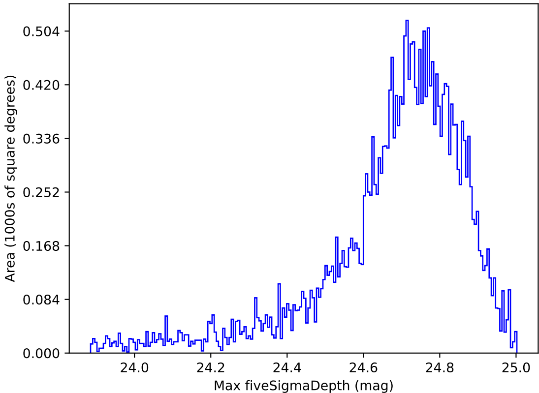
extra_ss_neo7_v3.4_10yrs All sky r band: Max fiveSigmaDepth
